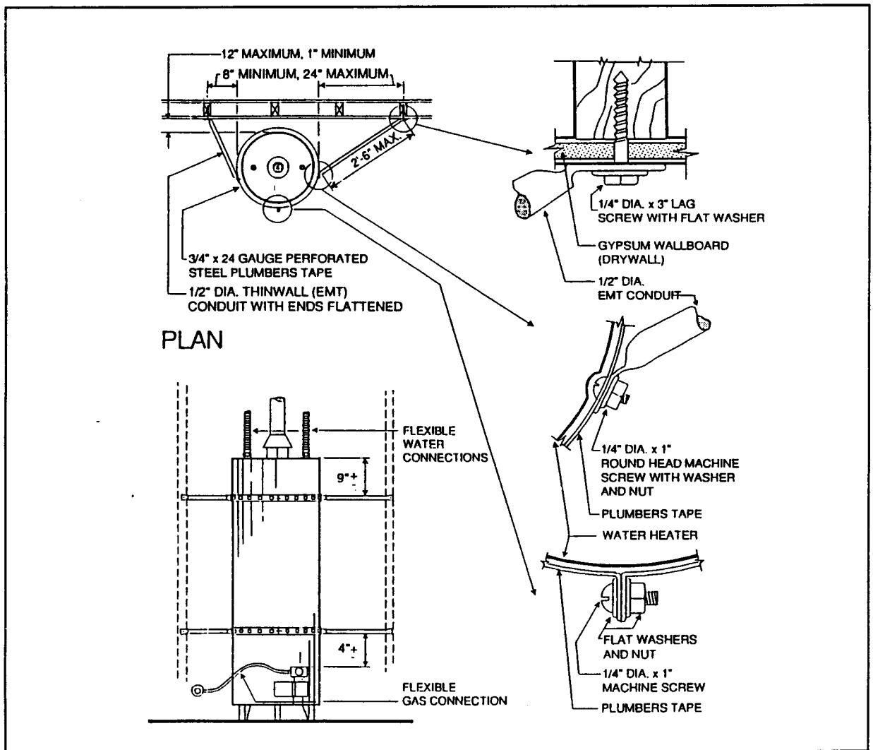
ELEVATION WATER HEATER ON STRAIGHT WALL
